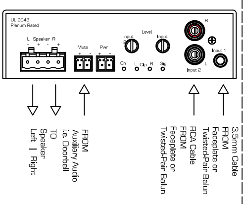
Enlarged View 1.1 [Back of Amplifier]
